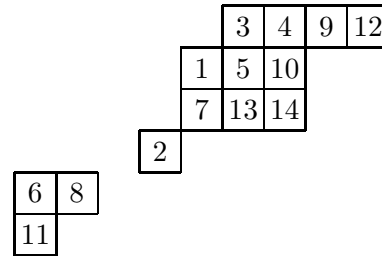
A standard tableau p of shape \lambda/\mu
