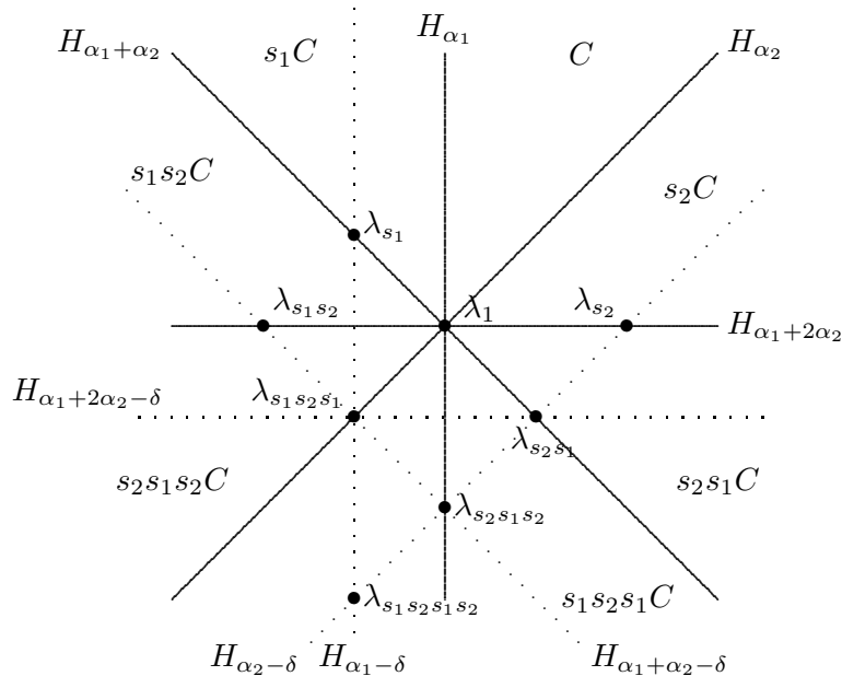
The arrangement \mathcal{A}^-
