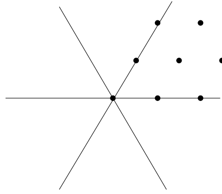
Cone of dominant integral weights
