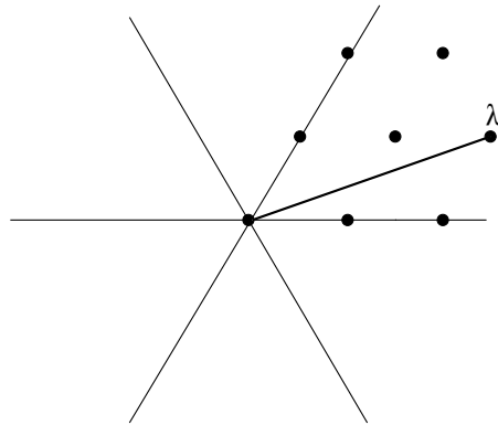
Path from 0 to \lambda
