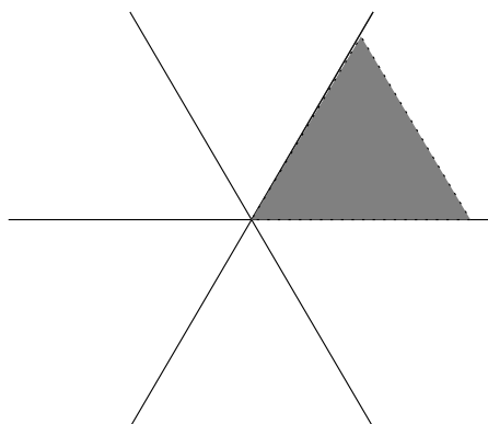
A chamber for A_2
