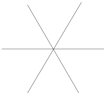
Hyperplane arrangement for A_2
