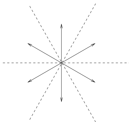
Root system for A_2
