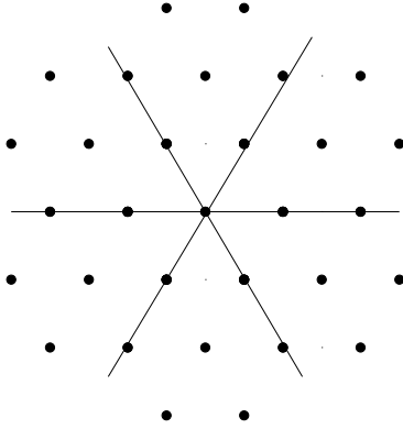
Lattice of integral weights
