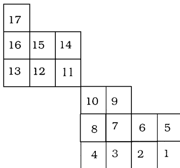
Figure 3. Filling for \mu = (2, 4, 4) and \lambda = (1, 3, 3) .
